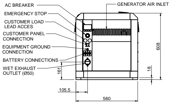
VIEW C
